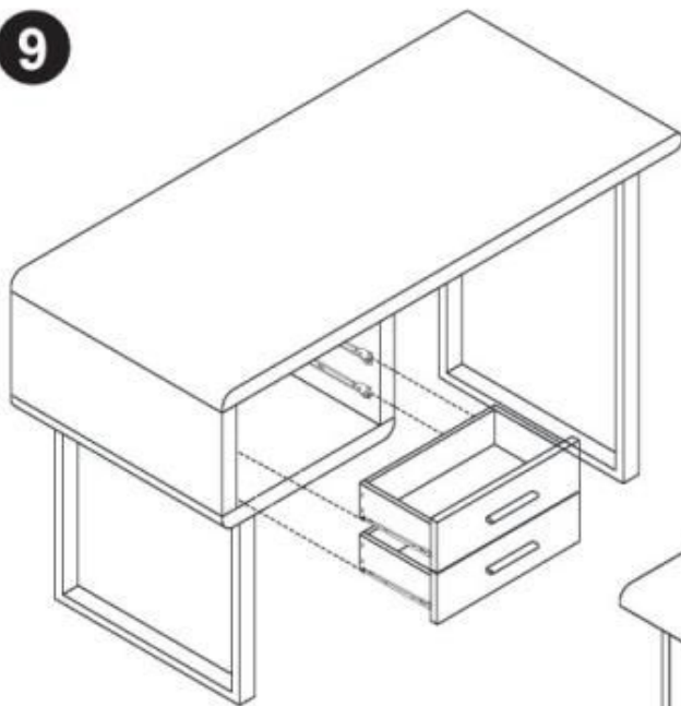
Left drawer assembly.
